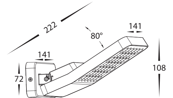
HV3721N-GRY Dimensions
