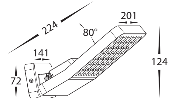
HV3722N-GRY Dimensions
